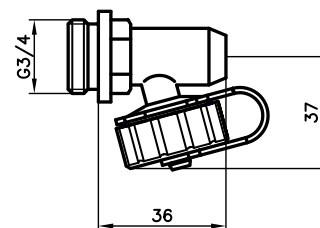
KFE-Hahn
